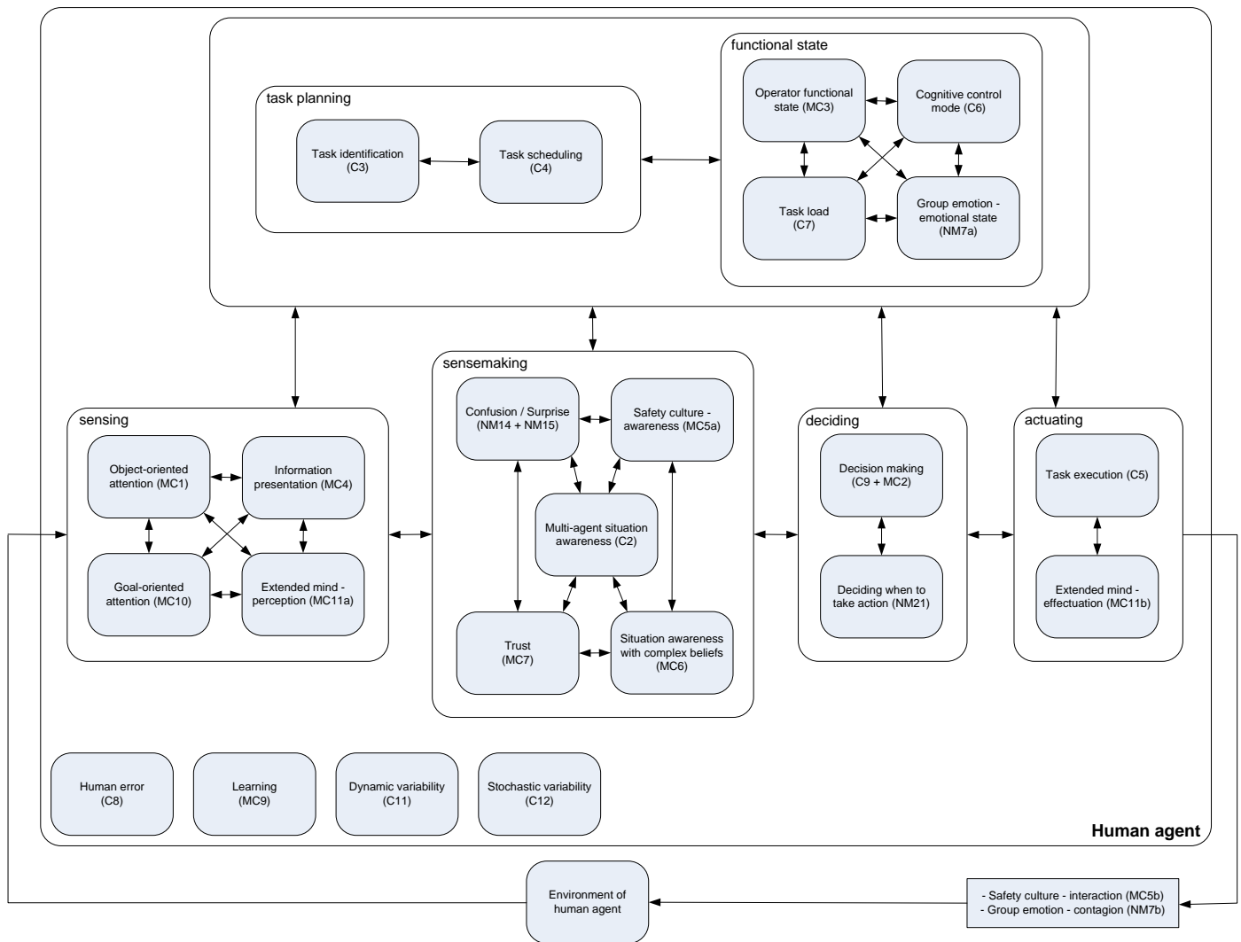
Figure 2. Overview of the integration of model constructs related to a human agent.
